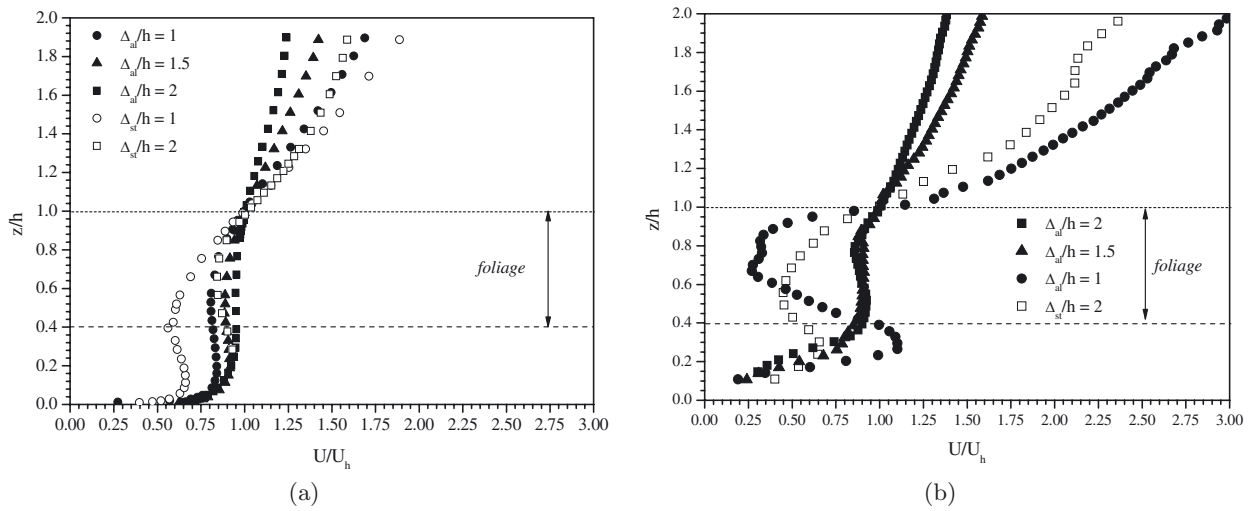
Fig. 2. Vertical profiles of the mean longitudinal velocity for all canopy densities and both configurations (a) Coniferous tree canopies (LDV measurements). (b) Round tree canopies (PIV measurements).
