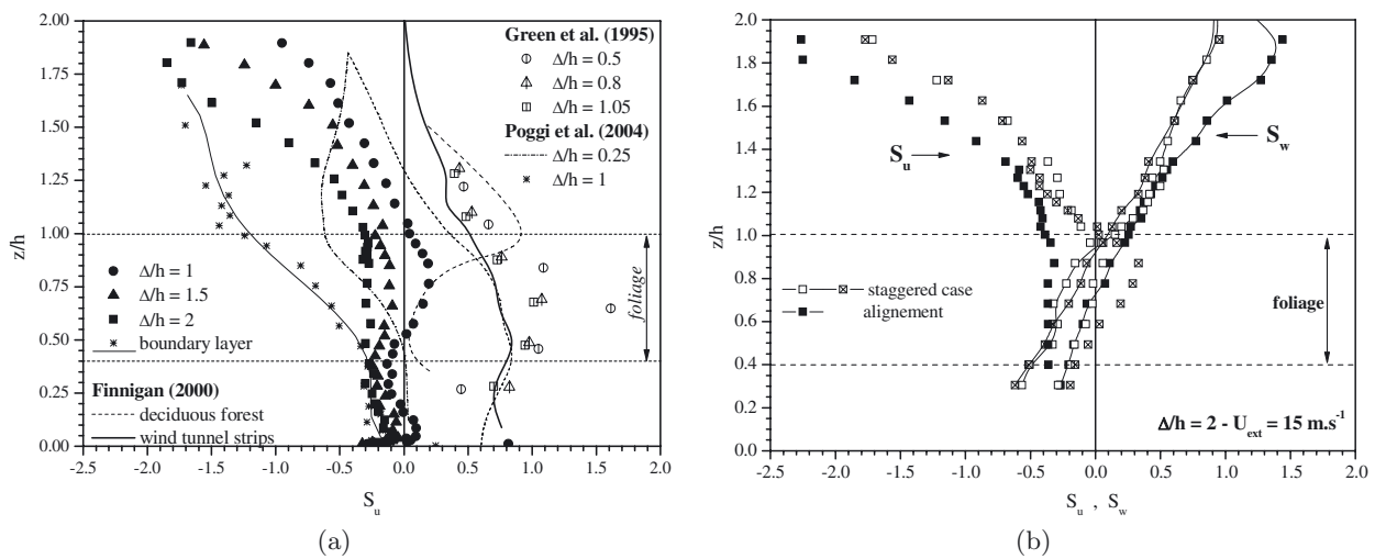
Fig. 3. Vertical profiles of velocity skewness, conifer canopies (a) longitudinal velocity; aligned arrangement (b) velocity longitudinal and vertical components; both spatial arrangements.
