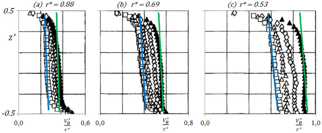
Fig. 8. Validation of Equations (10) and (11). Dimensionless tangential velocity profiles, G = 0.08 , Re = 1.47 \times 10^6 , Ro \approx 0.0167 . Experimental results extracted from Debuchy et al. [12]: \square h/H = 1.00 ; \blacktriangle h/H = 0.25 ; —: Equation (10) with K_p = 0.20 , \tilde{\alpha} = 1.78 and b = -0.12 . —: Equation (10) with K_p = 0.28 , \tilde{\alpha} = 1.85 and b = -0.08 .
