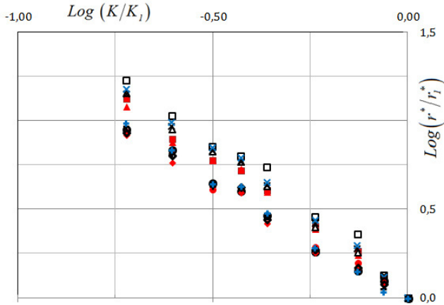
Fig. 3. Experimental validation of the behaviour law K/K_1 = (r^*/r_1^*)^{-\alpha} . Present experimental results extracted from Abdel Nour et al. [9]: see the symbols in Table 1.
