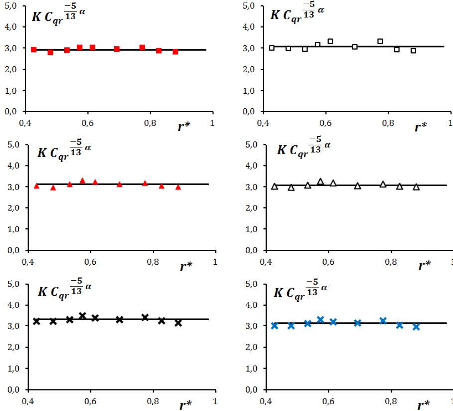
Fig. 4. Experimental validation of the behaviour law (7).
