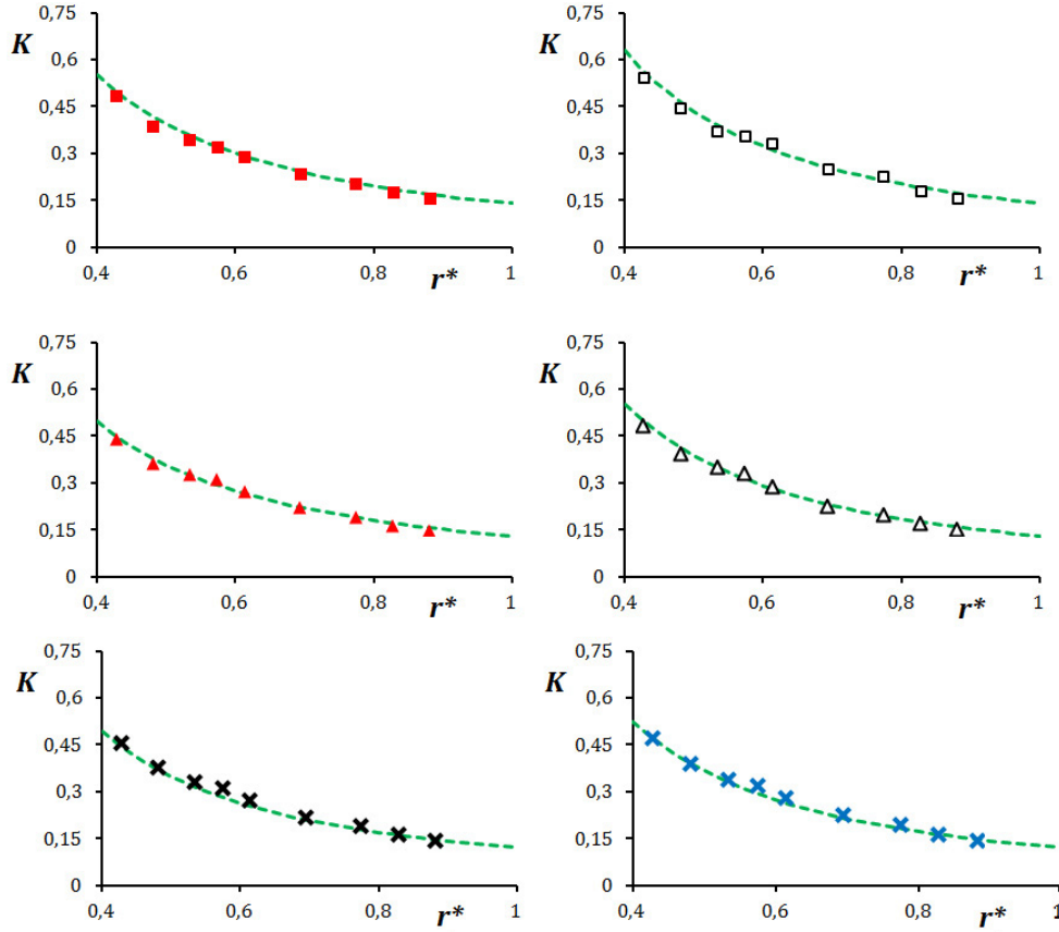
Fig. 5. Radial distribution of the core swirl ratio – G = 0.053 .
