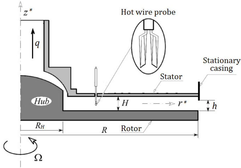
Fig. 1. Schematic diagram of the cavity.
