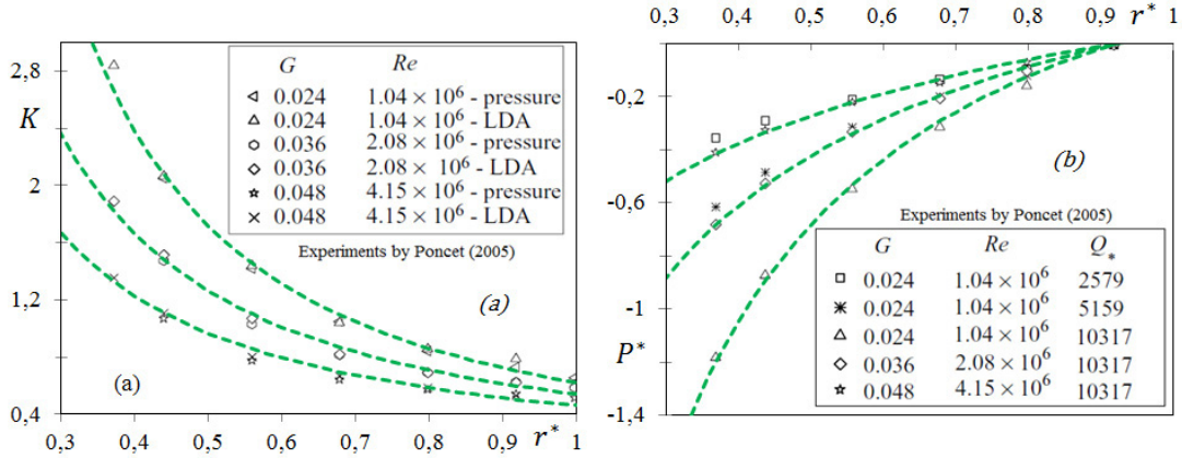
Fig. 9. Validation of the present behaviour law with the experiments by Poncet et al. [6]. ----: results from Equations (4) and (13) with the computed values of \tilde{\alpha} with Equation (12).
