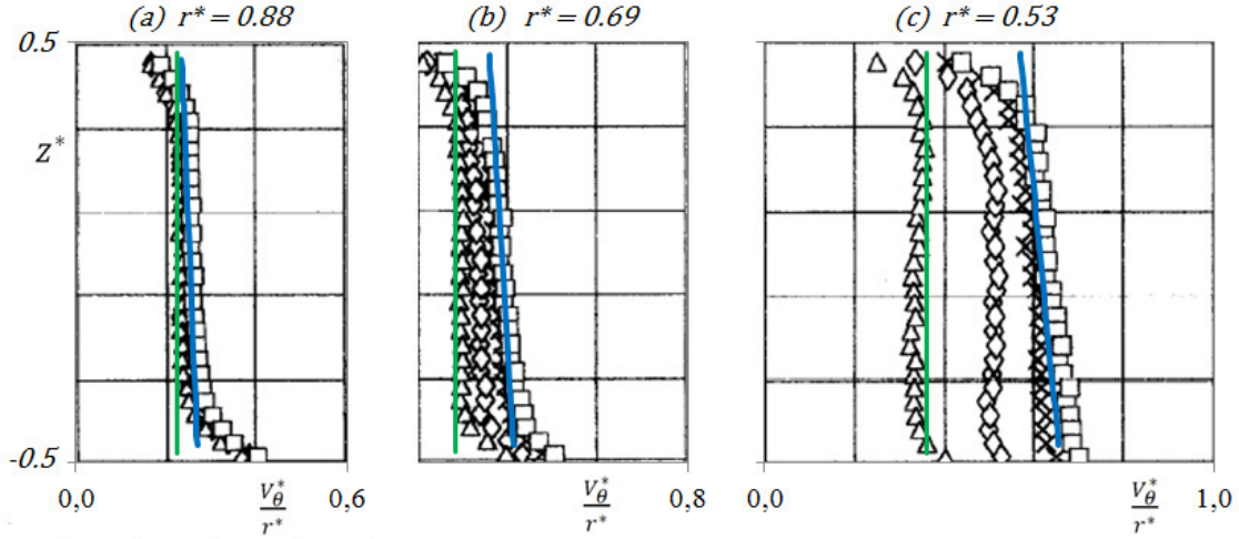
Fig. 7. Validation of Equations (10) and (11). Dimensionless tangential velocity profiles G = 0.08 , Re = 1.47 \times 10^6 , K_p = 0.20 . Experimental results extracted from Debuchy et al. [12]: \triangle isolated cavity, \square Ro \approx 0.0167 ; —: Equation (10) with \tilde{\alpha} = 1.78 and b = -0.12 ; —: Equation (11) with \tilde{\alpha}_0 = 0.94 .
