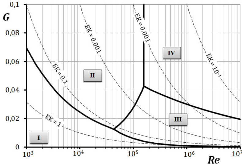
Fig. 2. Flow regimes according to the classification by Daily and Nece [13].
