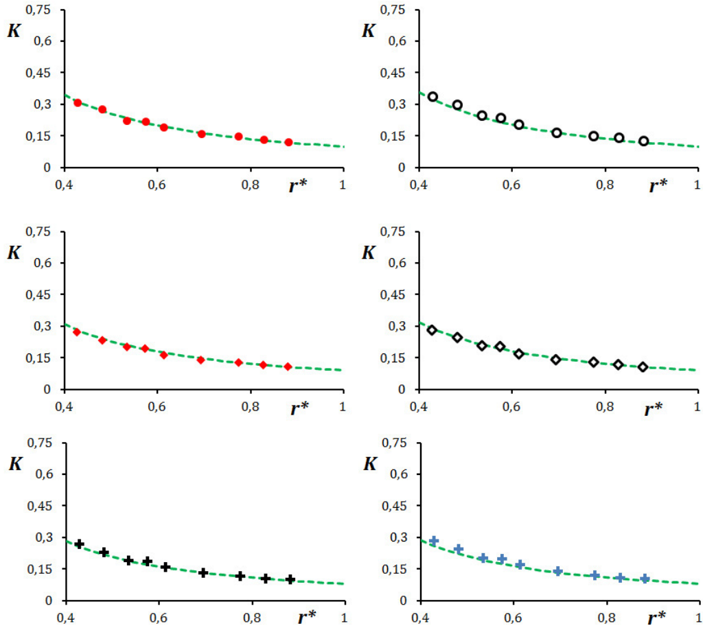
Fig. 6. Radial distribution of the core swirl ratio - G = 0.08 . Experimental results extracted from Debuchy et al. [16]: see the symbols in Table 1; ----: Equation (4) with the computed values of \tilde{\alpha} according to Equation (8).
