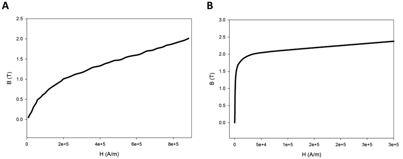
Fig. 1. B-H curves for: (a) MRF-132DG [29], (b) steel 1018 [21].
